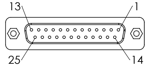
Female Connector
