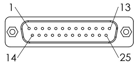
Male Connector
