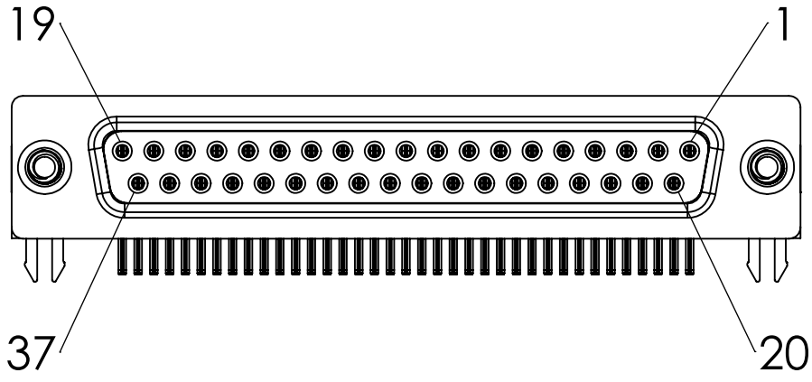
Connector Pinout (Female)
